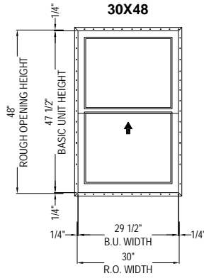
50/50 Sash Split 30 CALLOUT WIDTH
