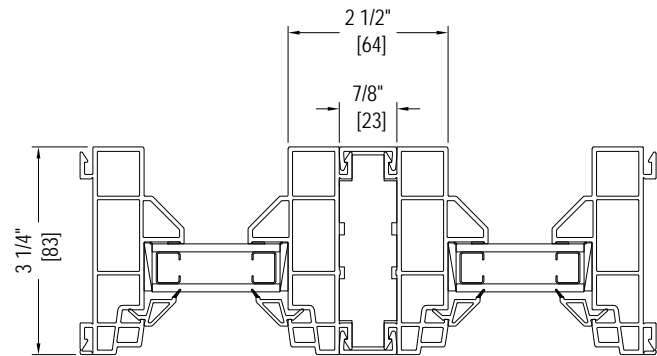
MULL DETAIL SUPERSEAL DIRECT SET / DIRECT SET
