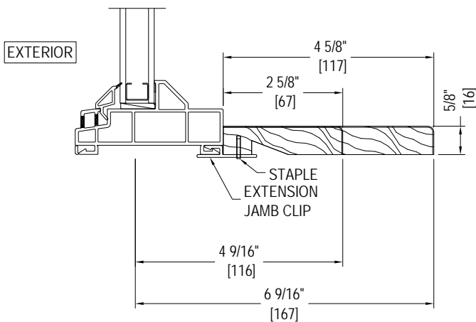
EXTENSION JAMB DETAILS
