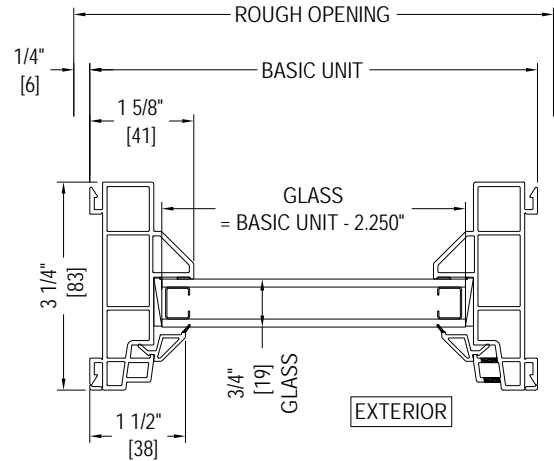
JAMB DETAIL SUPERSEAL DIRECT SET
